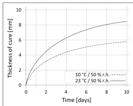
Diagram 1: Curing speed Sikaflex®-545
