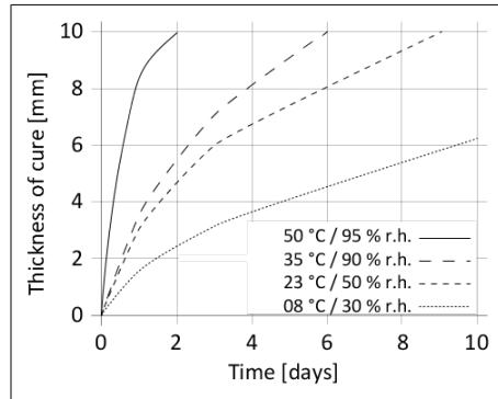
Diagram 1: Curing speed Sikasil® AS-165
