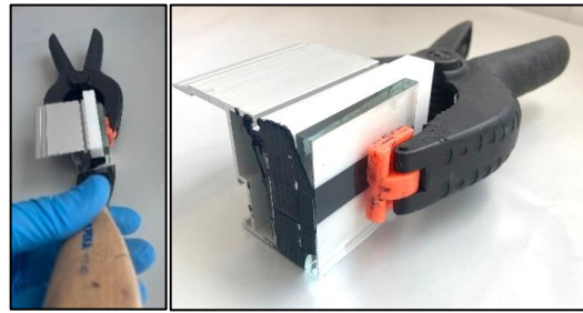
Figure 24: Remove excessive adhesive to ensure a proper, smooth and uniform adhesive surface
