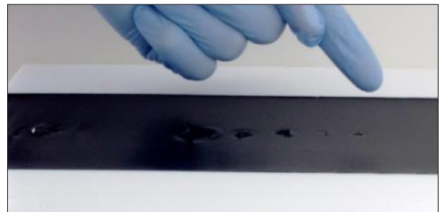
Figure 18: If no residues on your fingers are recognized the skin-over time has been reached
