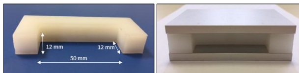
Figure 32: Alternative test arrangement (suitable for profiles and 1-component adhesive)
