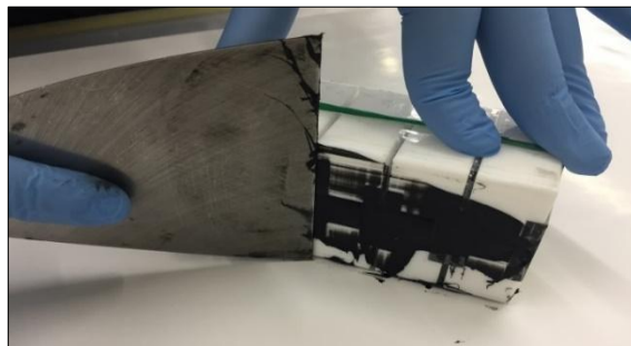
Figure 30: Remove excessive adhesive to ensure a proper, smooth and uniform adhesive surface
