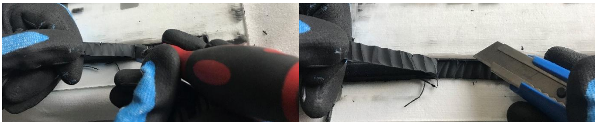
Figure 20: Peel adhesion test on float glass: cutting the bead while pulling
