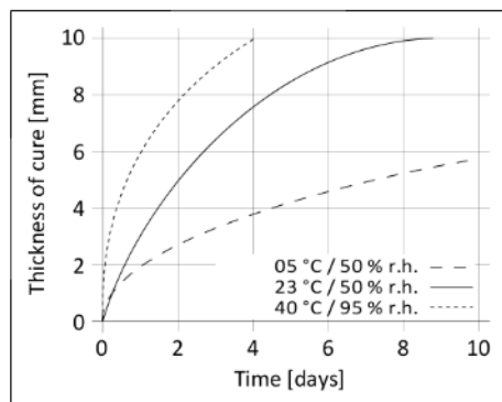
Diagram 1: Curing speed Sikasil® AS-65
